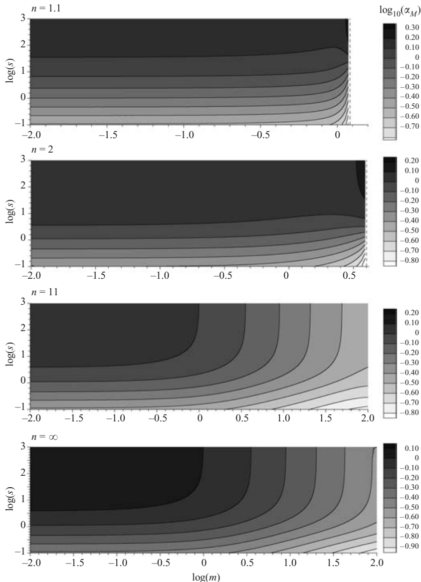
FIGURE 6. Contour plots of \alpha_M corresponding to \gamma_M of figure 5.
